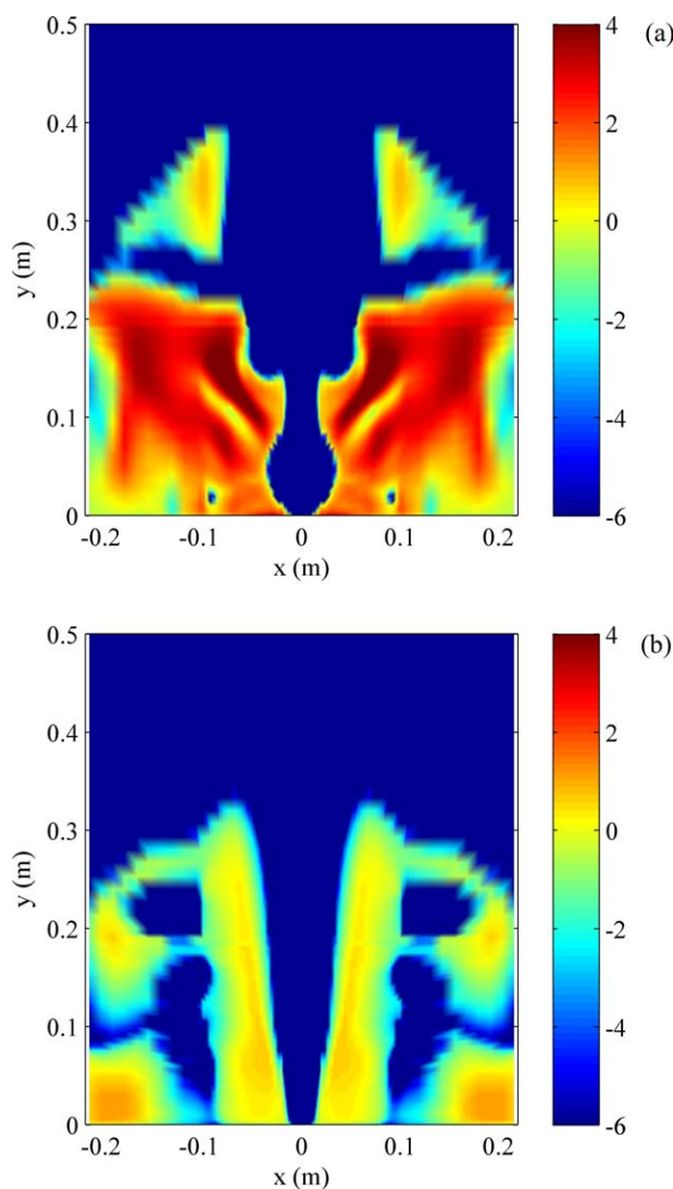
Figure 9. Frictional viscosity values on a log scale for V_f=V_{mf} at t=15 s.
