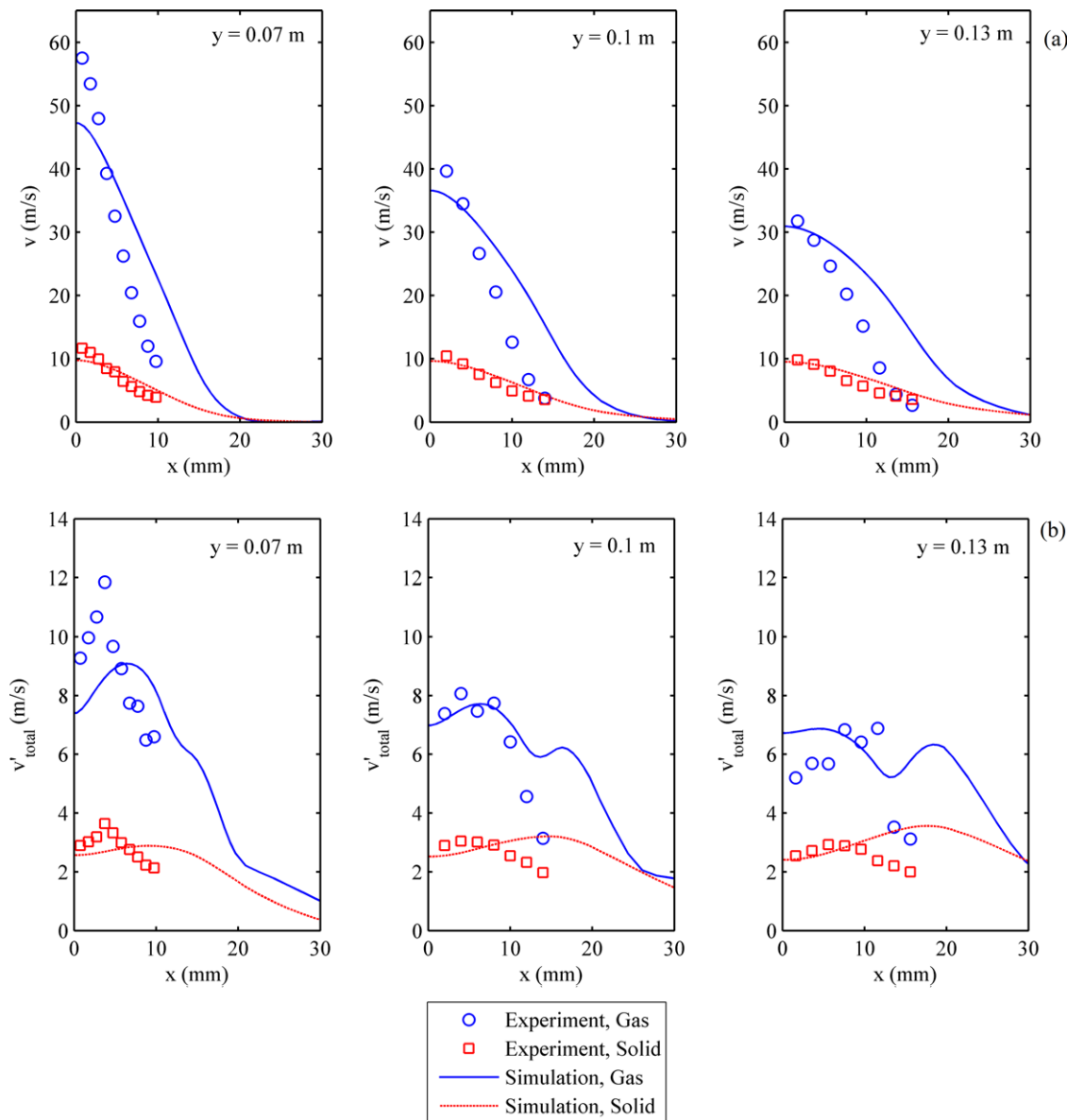
Figure 13. Streamwise velocity profiles for V_{fl}=0.7 V_{mt} .
