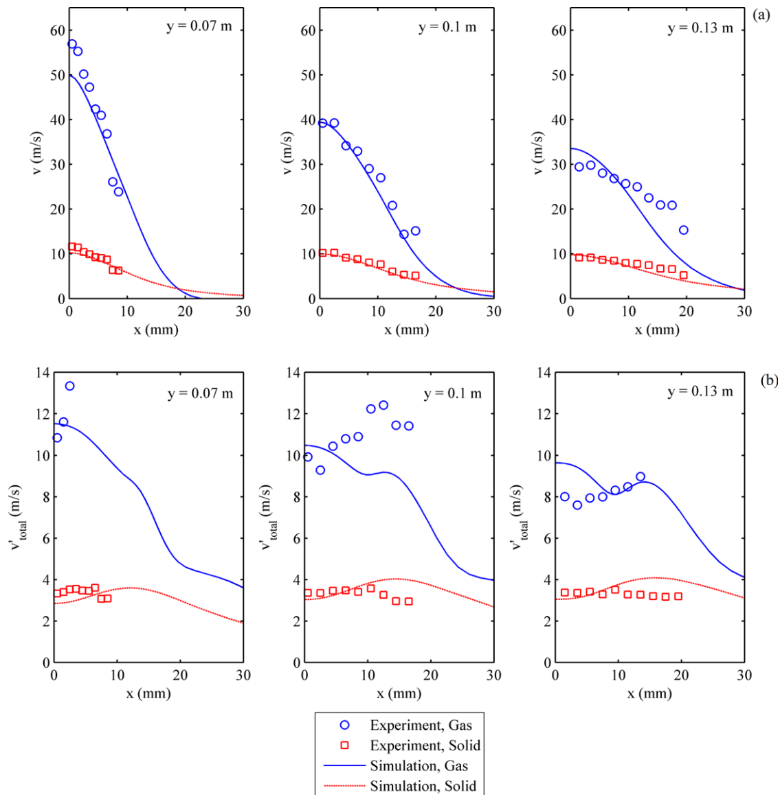
Figure 15. Streamwise velocity profiles for V_{fi}=1.3 V_{mf} .
