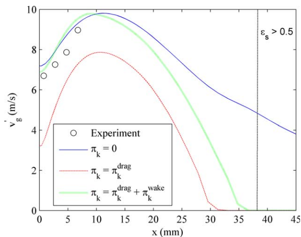
Figure 10. Influence of gas turbulence modulation term on the gas fluctuating velocity at y=0.1 m for V_f=0 .
