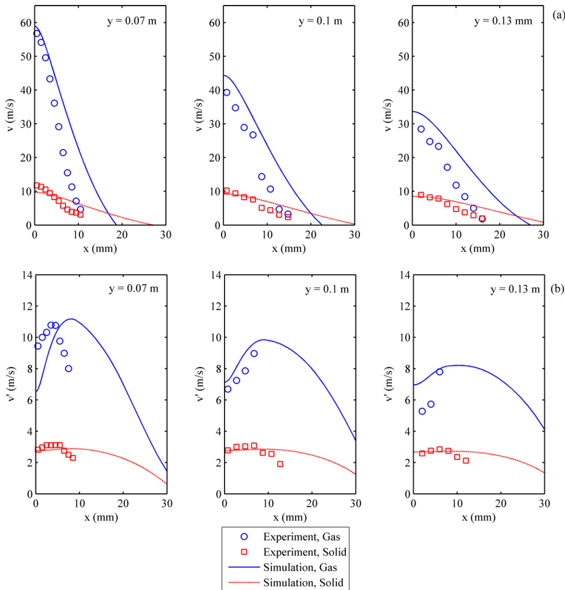
Figure 12. Streamwise velocity profiles for V_f=0 .
